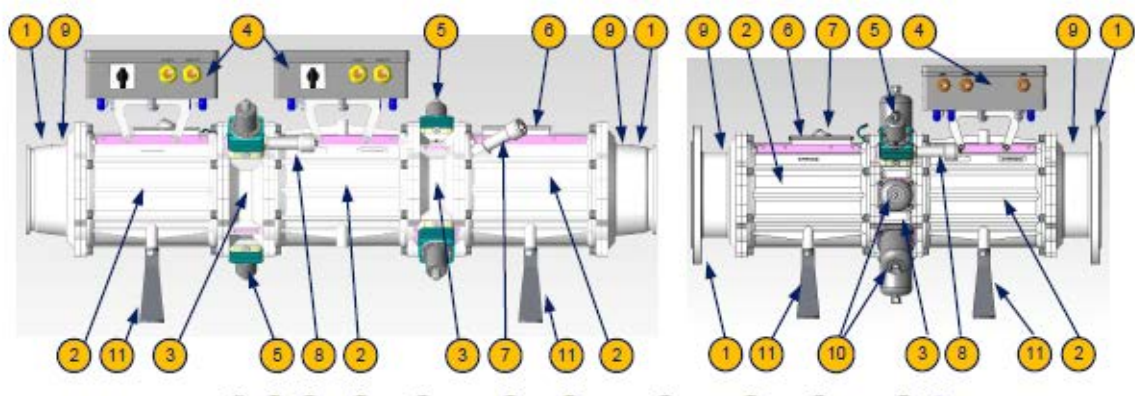
Figure 2-1: RZ163-12, RZ163-11 Units.
