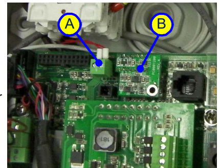
Figure 10-35: Location of the Temperature Sensor Connector (Generic)
