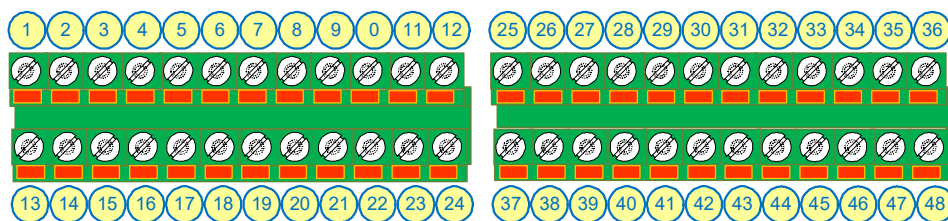
Figure 5-30: Control Module Terminal Connectors
