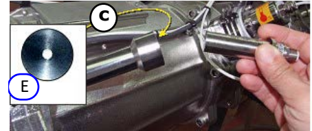
Figure 10-32: Replacing the Sensors 3 (Generic View)
